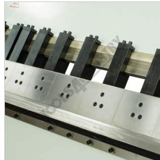
Removable Fingers
