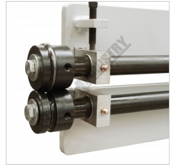
Bearing Guide Block with Grease Nipples
