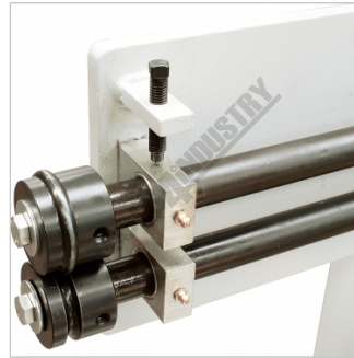
Top Roll Adjusting Screw
