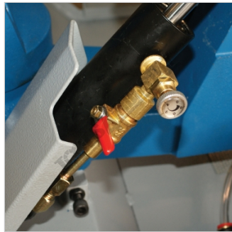
Hydraulic Down Feed Control
