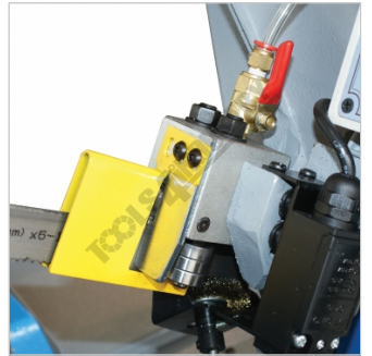
Ball Bearing Blade Guides - Back
