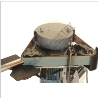
Tilting Table for Contouring & Pipe Notching
